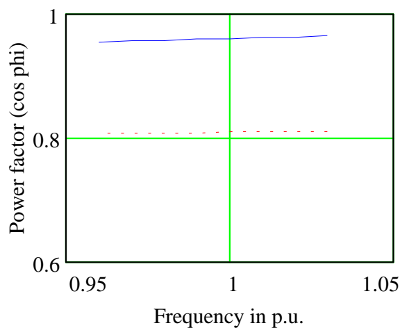
Figure 34. The power factor ( \cos \varphi ) versus the frequency f in p.u. Solid curve: with reactive power compensation. Dotted curve: without reactive power compensation. P = 225 \text{ kW} and U = 400 \text{ V} in all points.
