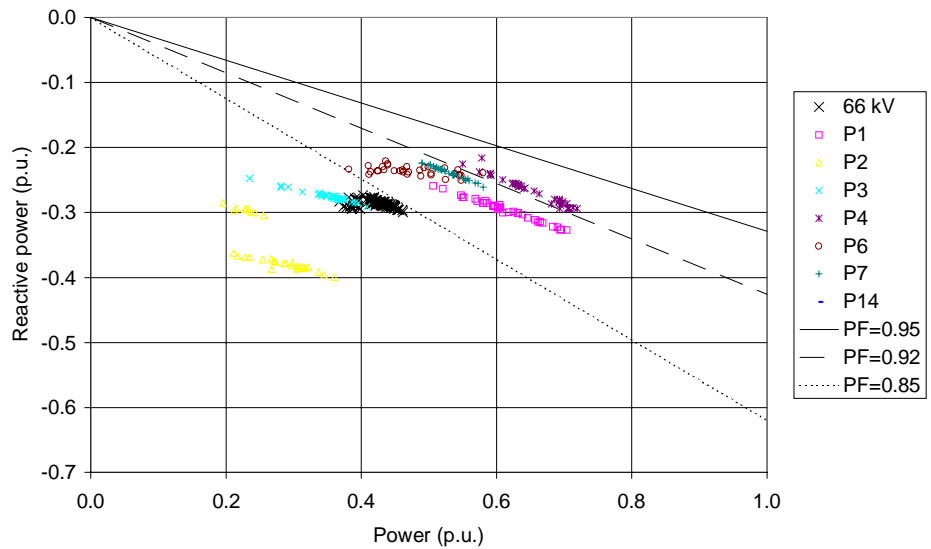
Figure 7. Feederwise reactive power consumption in the Lamba substation
