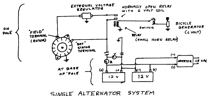
SINGLE ALTERNATOR SYSTEM
