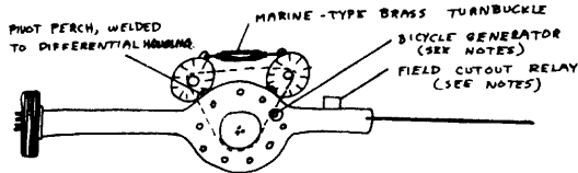
TOP VIEW 2 ALTERNATOR UNIT
