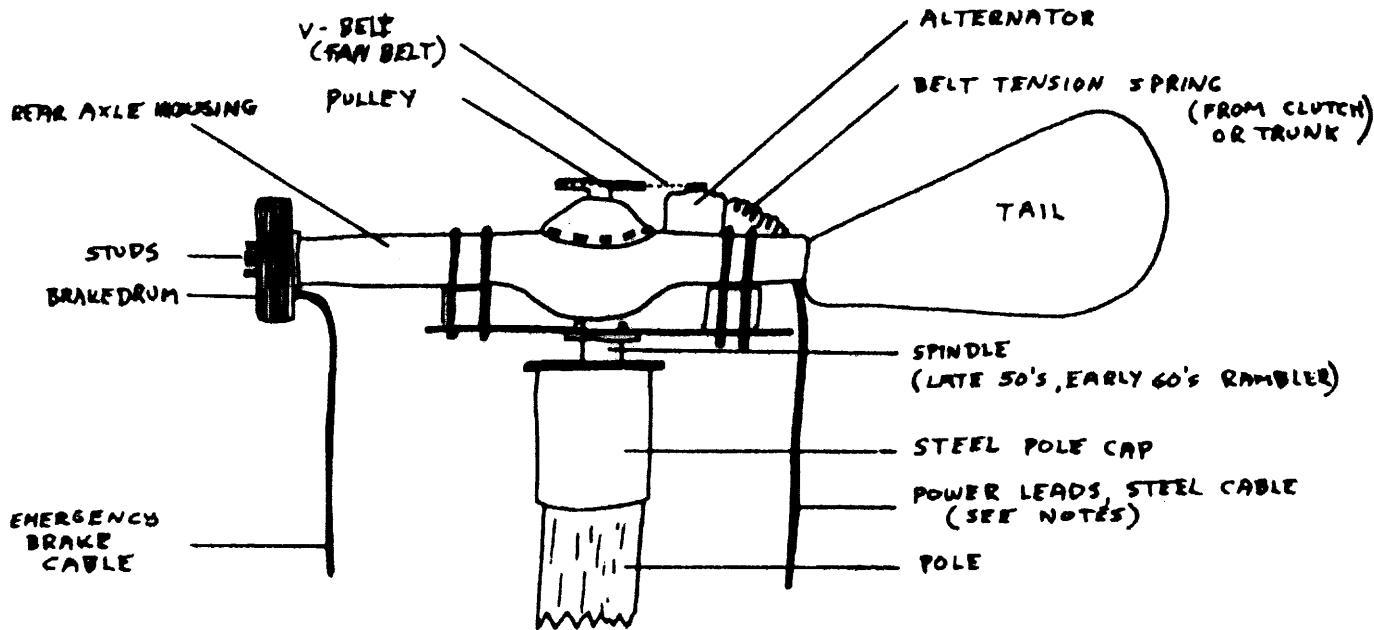
SIDE VIEW SINGLE ALTERNATOR UNIT
