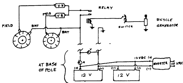
2 ALTERNATOR SYSTEM
