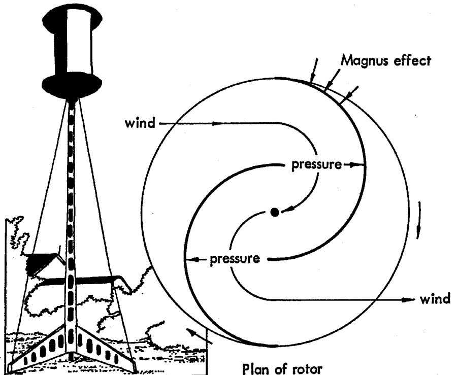
Captain Savonius' wind motor built in Helsinki in 1924; with diagrammatic plan of the rotor arrangement. Adapted from G. Bathe, Horizontal Windmills, Draft Mills and Similar Air-flow Engines , Allen, Lane and Scott, Philadelphia 1948 Plate XVII
